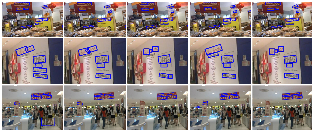
FIGURE 7. The fusion of multi-oriented bounding boxes detected by deep learning-based methods. The first four columns illustrate detection results achieved by the Pelee-Text, TextBoxes++, PixelLink, and PSNet networks, respectively, and the last column shows the performance results achieved by our GP-based fusion method.
